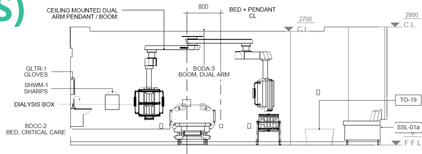
3 (ICU 03)-ELEVATION-S 1:50
