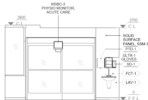
4 (ICU 03)-ELEVATION-W 1:50
