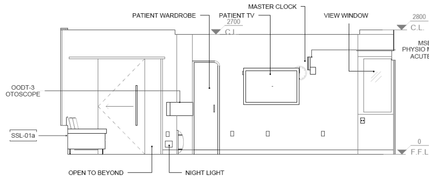
2 (ICU 03)-ELEVATION-N 1:50
