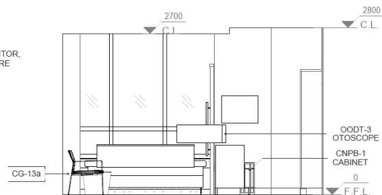
1 (ICU 03)-ELEVATION-E 1:50
